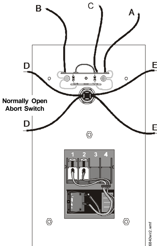
BG-12LRA (rear view) Agent Release Pull Station
