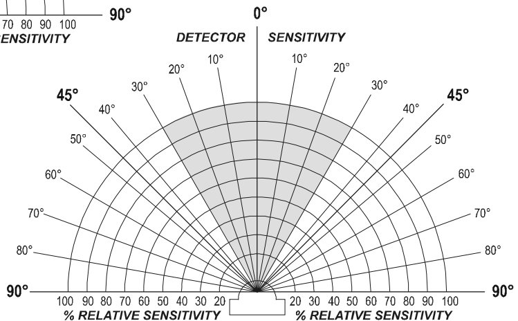
Figure 3 (above): Model 30-2021-24 Figure 4 (at right): Model 30-2021E-24 Viewing Patterns for Cone of Vision
