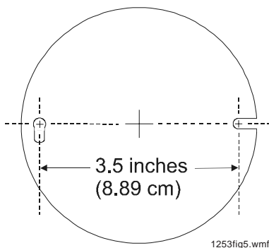
Figure 5: Model 30-2021-24 Mounting Holes
