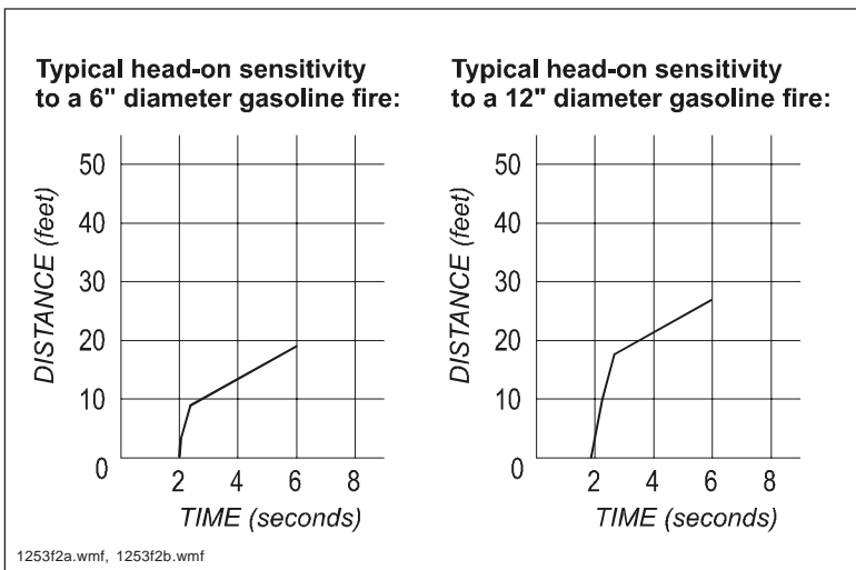
Figure 2: Model 30-2021E-24 Detector Sensitivity
