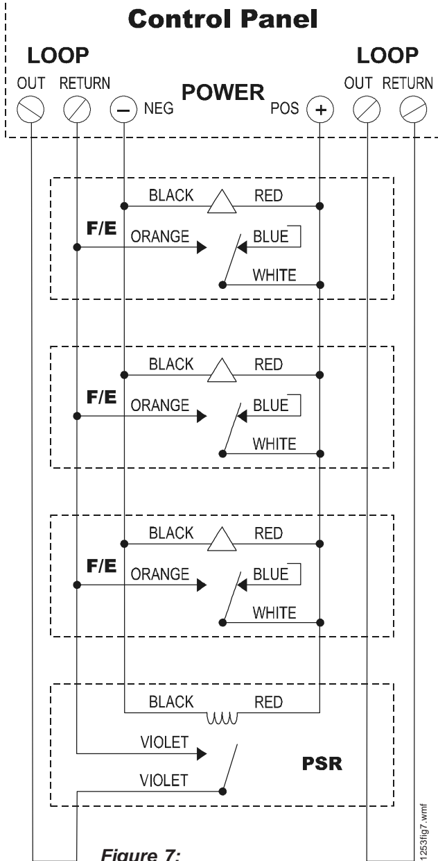
Figure 7: Double-Loop Panel Wiring
