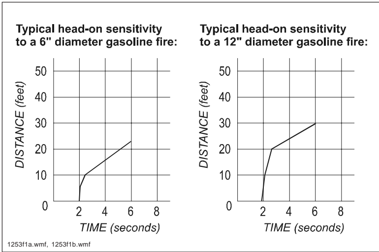
Figure 1: Model 30-2021-24 Detector Sensitivity
