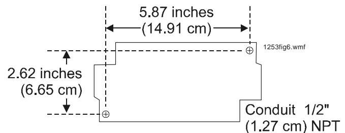
Figure 6: Model 30-2021E-24 Mounting Holes
